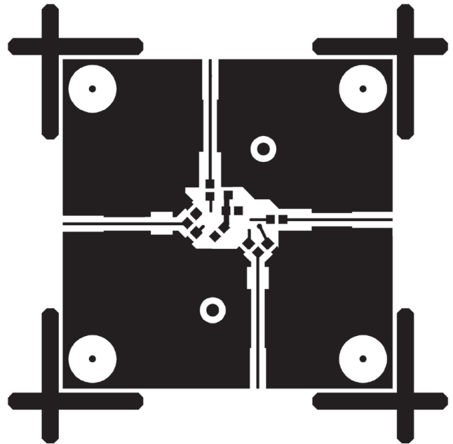
Figure 15. MSOP Evaluation Board, Amplifier Side (Bottom)
